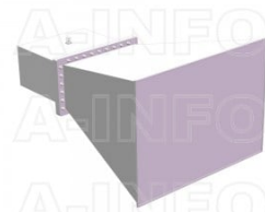
LB-1800-10-C-7/16FSPO Standard Gain Horn Antenna 0.41-0.62GHz 10dB Gain 7/16(DIN) Female
